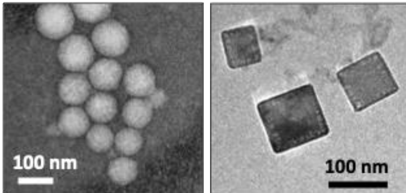
Polymer-based nanomaterials
